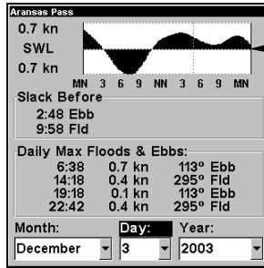
Current Information screen.
